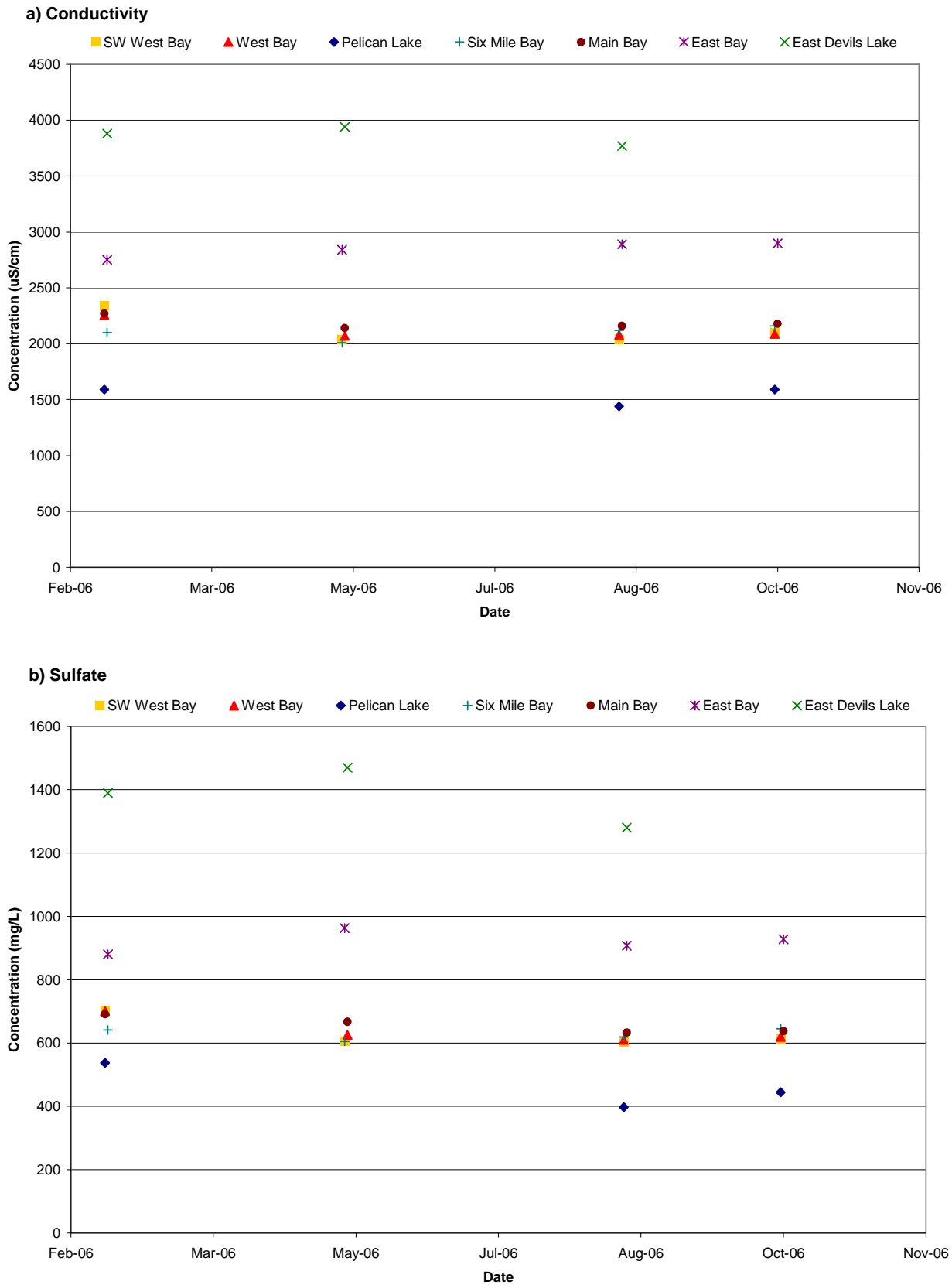
Figure 4. Surface Concentrations (Collected at 1 Meter) of Selected Parameters and Secchi Disk Transparency for Each Devils Lake Sampling Site and Event in 2006
