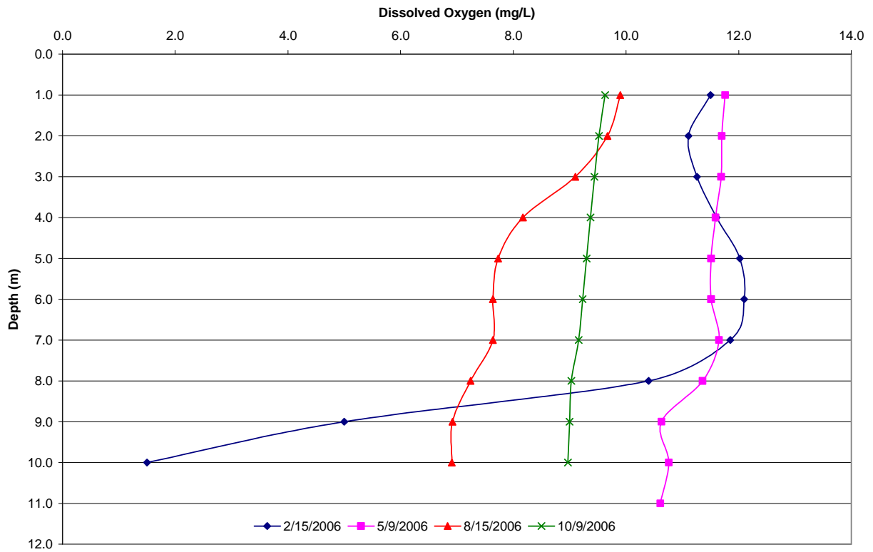
Figure 6. Temperature and Dissolved Oxygen Profiles for Devils Lake Sampling Sites and Events in 2006
